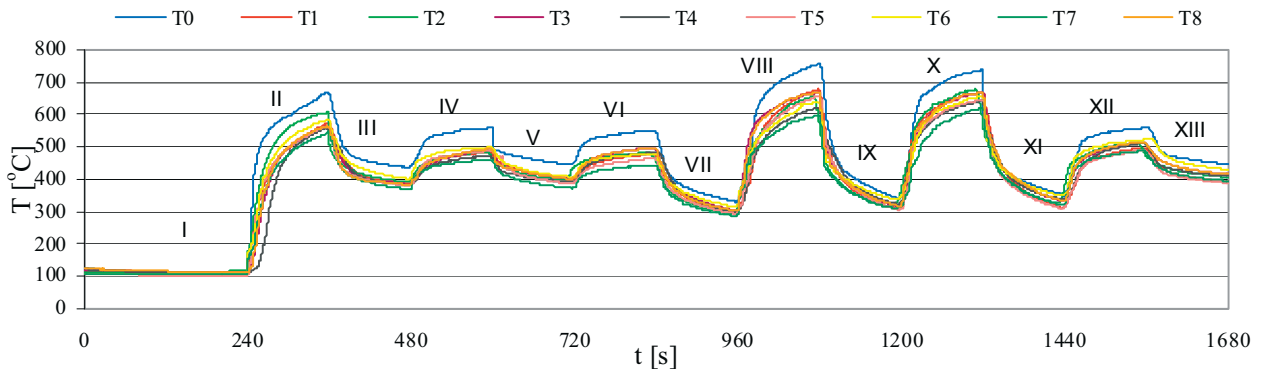
Fig. 8. Distribution of temperature in measurement point T0-T8 exhaust pipe of testing engine without catalytically converter during realization ESC test [6]
