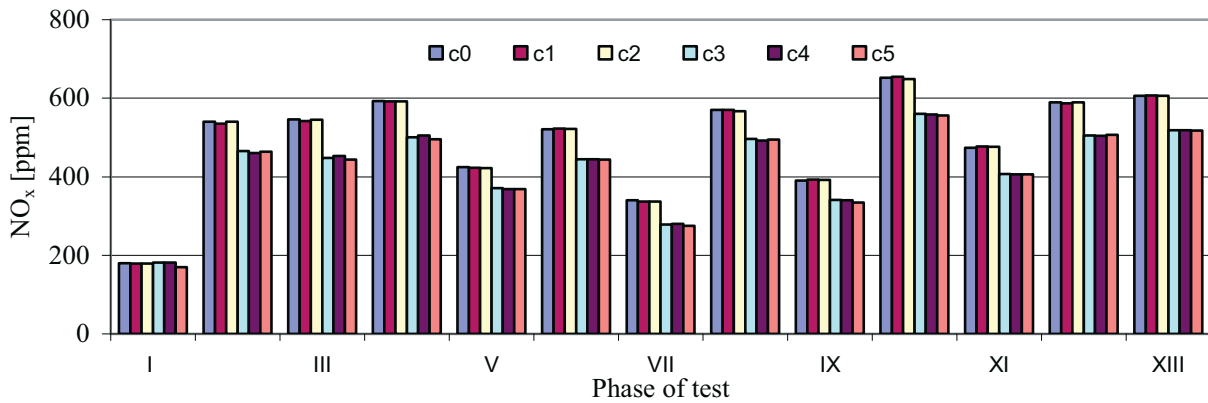
Fig. 13. Value of NO x concentration during ESC test of catalytically converter with 200 cpsi [6]
