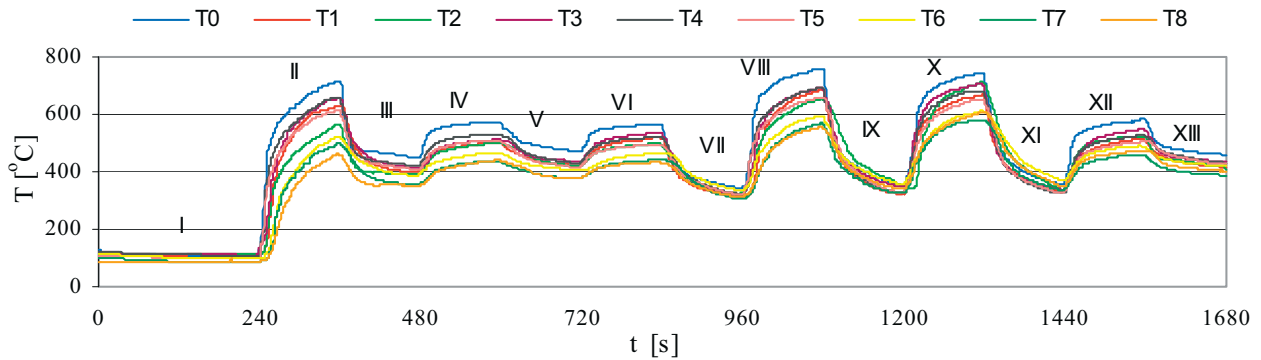
Fig. 9. Distribution of temperature in measurement point T0-T8 exhaust pipe of testing engine with 200 cpsi catalytically converter during realization ESC test [6]
