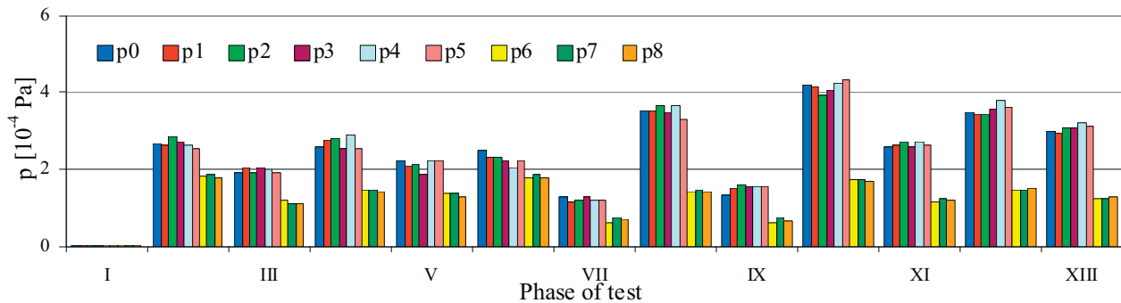
Fig. 10. Distribution of pressure in measurement point p0-p8 exhaust pipe of testing engine without catalytically converter during realization ESC test [6]
